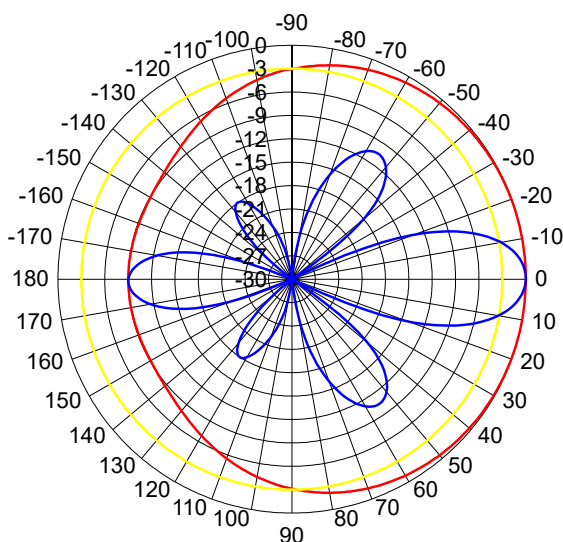
RADIATION PATTERN
